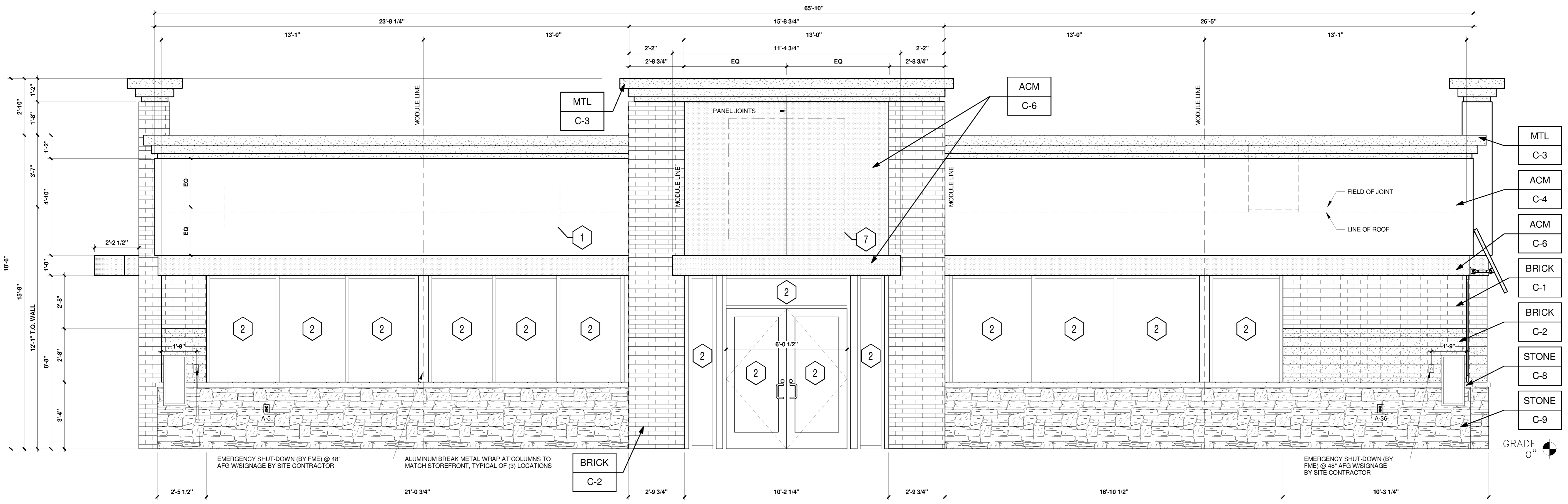
1 SOUTH-EAST ELEVATION 3/8" = 1'-0"
