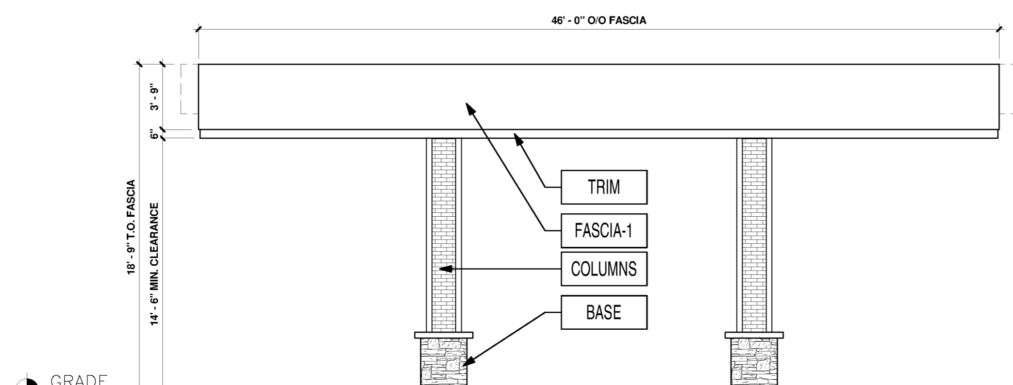
3 NORTH-EAST ELEVATION 3/16" = 1'-0"
