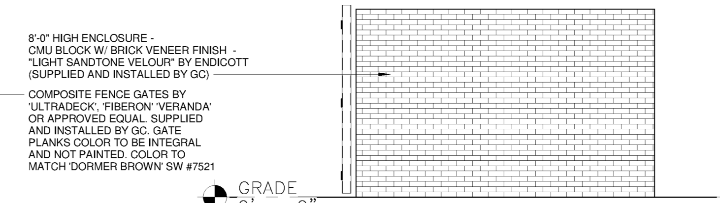
6 DUMSTER ENCLOSER - RIGHT ELEVATION 1/4" = 1'-0"
