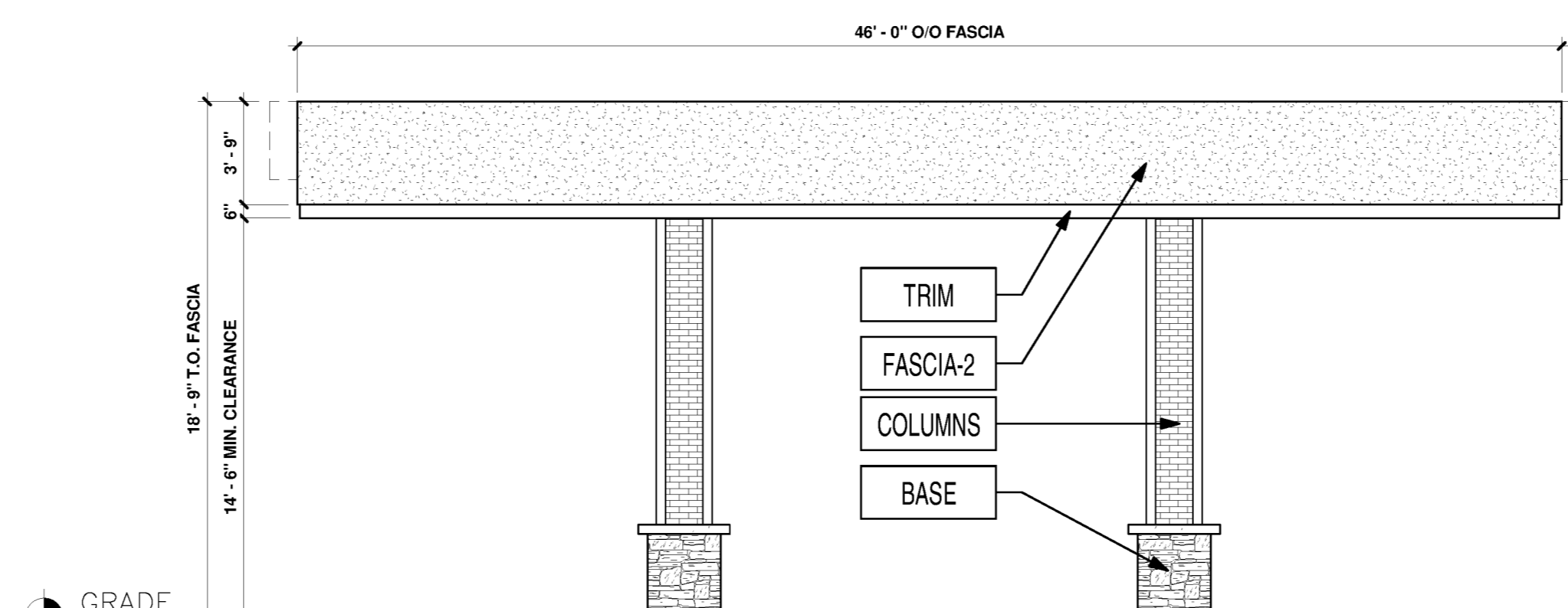
4 SOUTH-WEST ELEVATION - FOUNDERS PKWY 3/16" = 1'-0"
