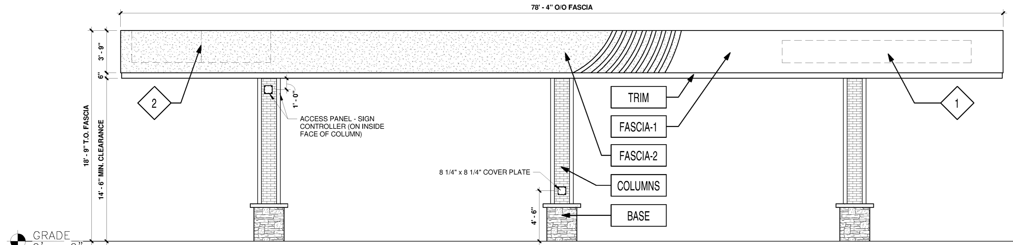
1 SOUTH-EAST ELEVATION 3/16" = 1'-0"
