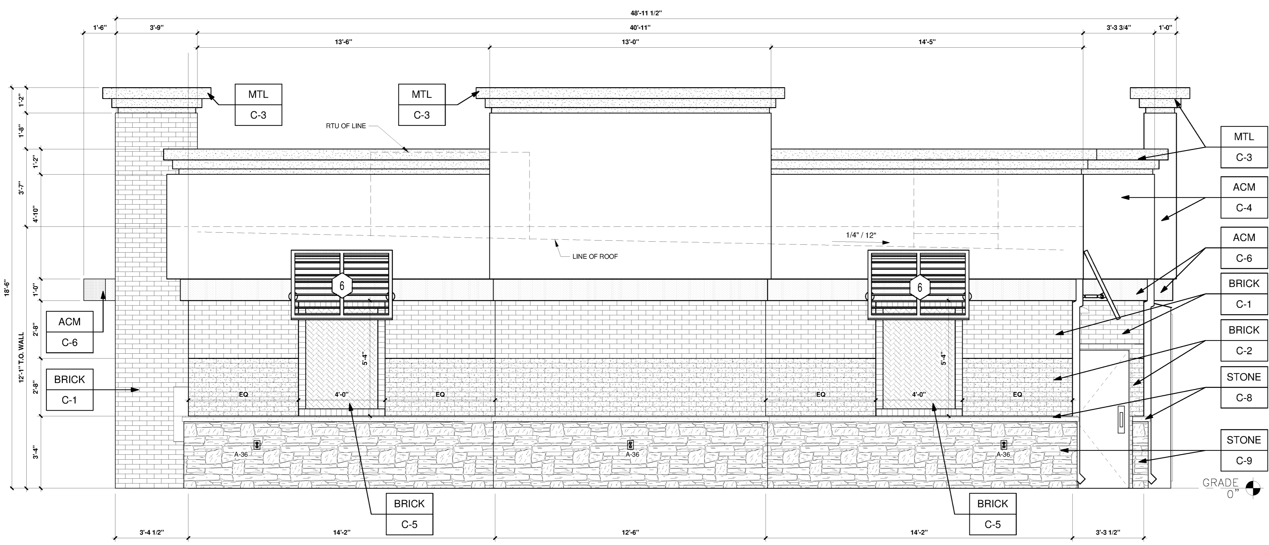
2 NORTH-EAST ELEVATION 3/8" = 1'-0"
