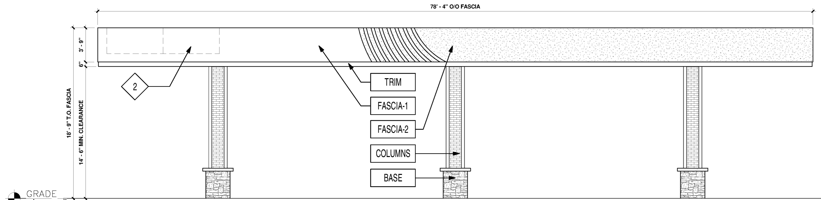
2 NORTH-WEST ELEVATION - METZLER WAY 3/16" = 1'-0"
