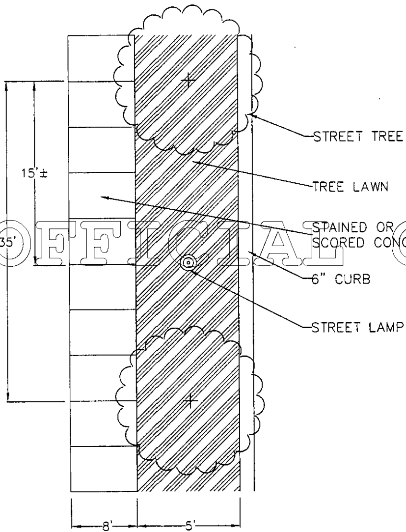
TOWN CENTER TYPICAL SIDEWALK TREATMENT AT LOCAL COLLECTOR
