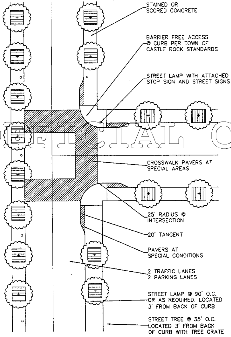
TOWN CENTER THREE WAY INTERSECTION WITH NECKDOWNS
