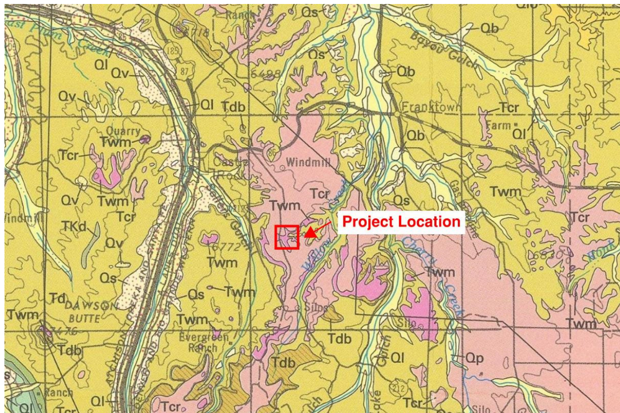
Figure 3-1. Geologic Map
