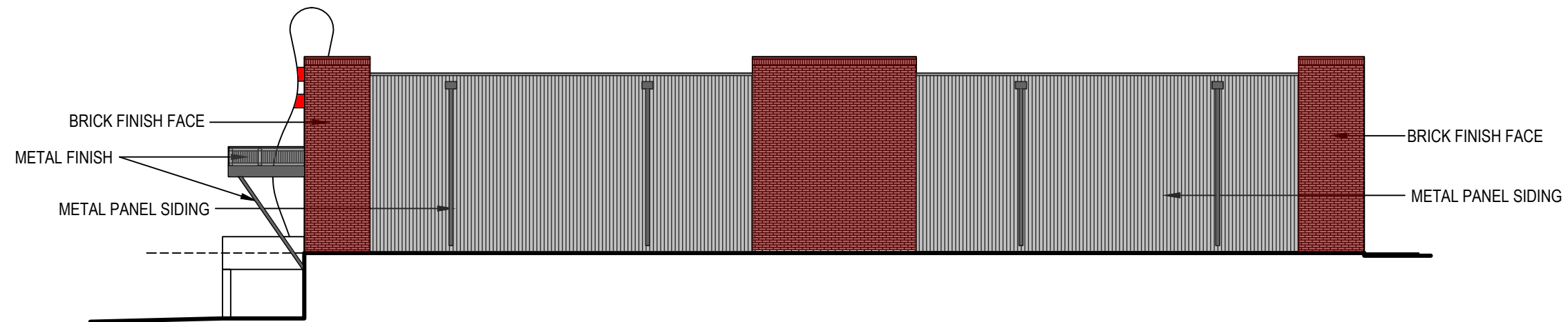
BUILDING #7 - NORTH ELEVATION
