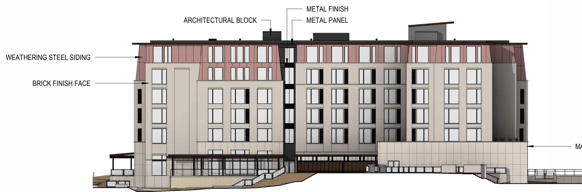
BUILDING 2 - EAST ELEVATION
