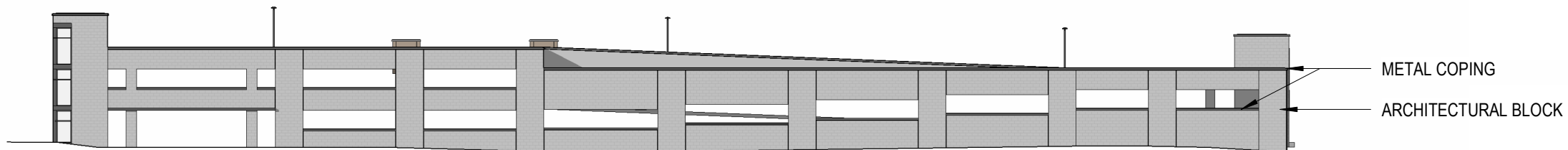
BUILDING 3 - EAST ELEVATION
