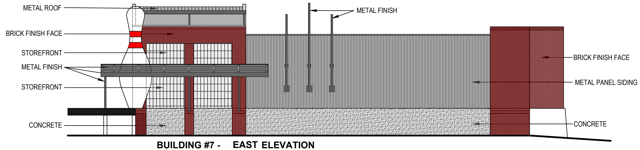
BRICK FINISH FACE COLOR: RED GALVALUME
