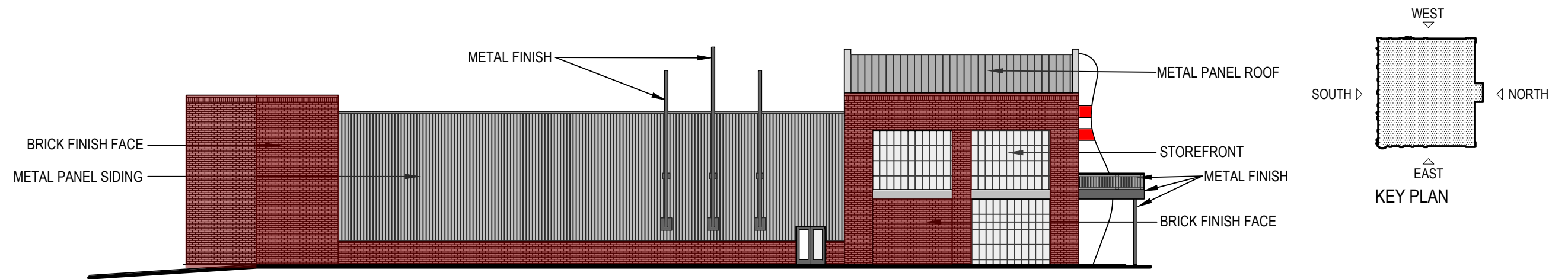
BUILDING #7 - WEST ELEVATION
