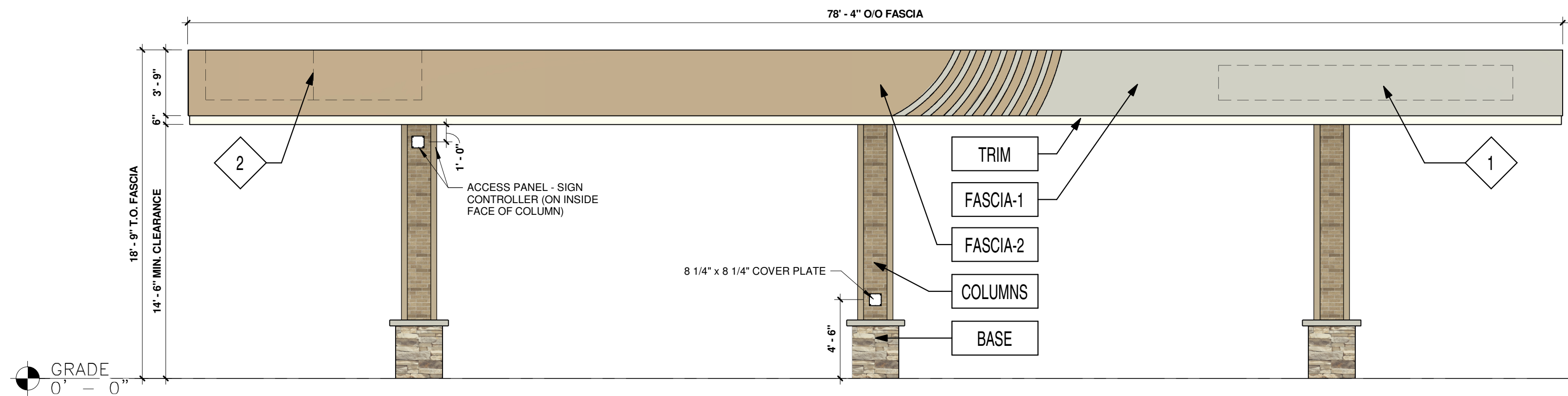
1 SOUTH-EAST ELEVATION 3/16" = 1'-0"
