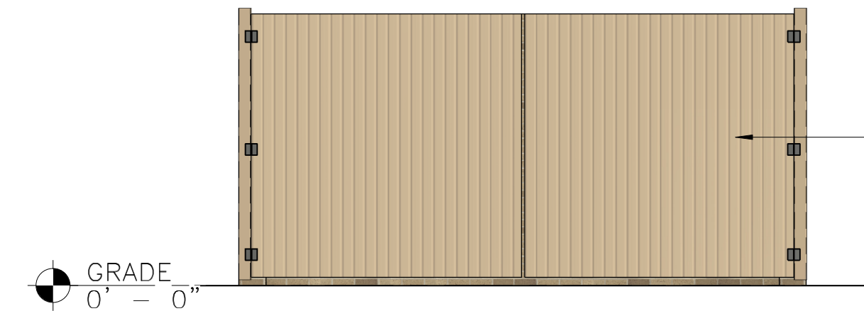
5 DUMSTER ENCLOSER - FRONT ELEVATION 1/4" = 1'-0"
