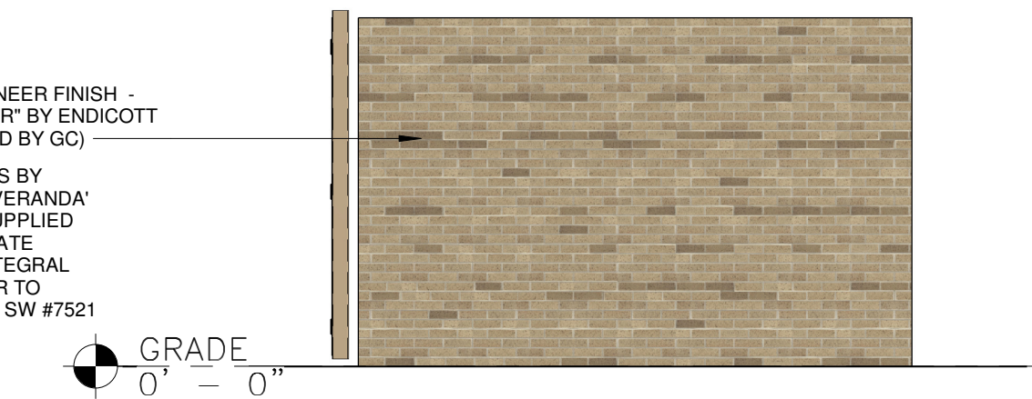
6 DUMSTER ENCLOSER - RIGHT ELEVATION 1/4" = 1'-0"
