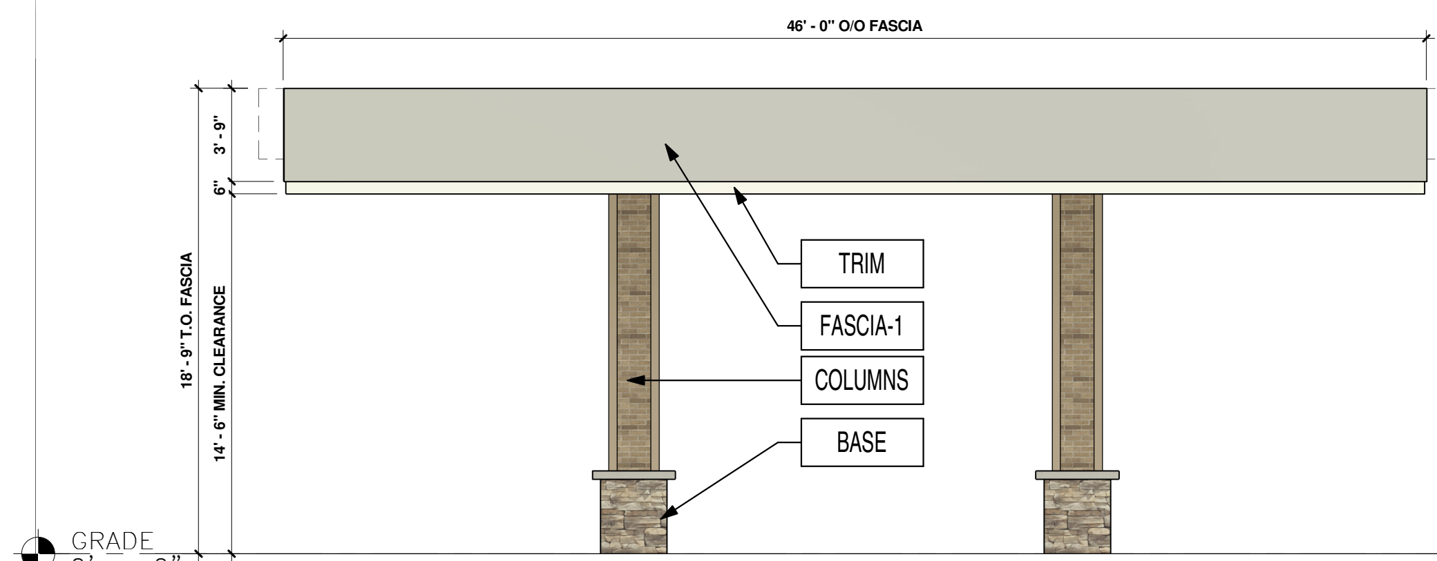
3 NORTH-EAST ELEVATION 3/16" = 1'-0"
