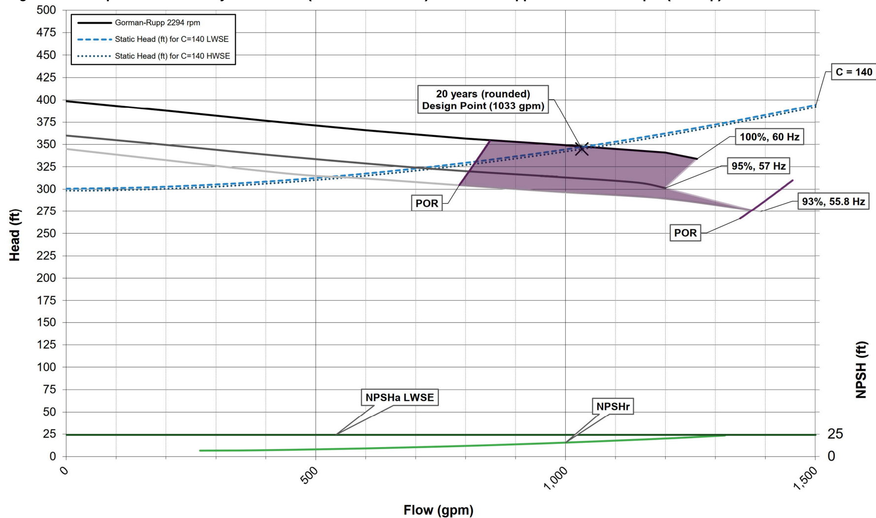
Figure 3.2: Pump Selection for 20-year Buildout (Future Conditions) – Gorman Rupp 6504E60-B 2294 rpm (1 Pump)
