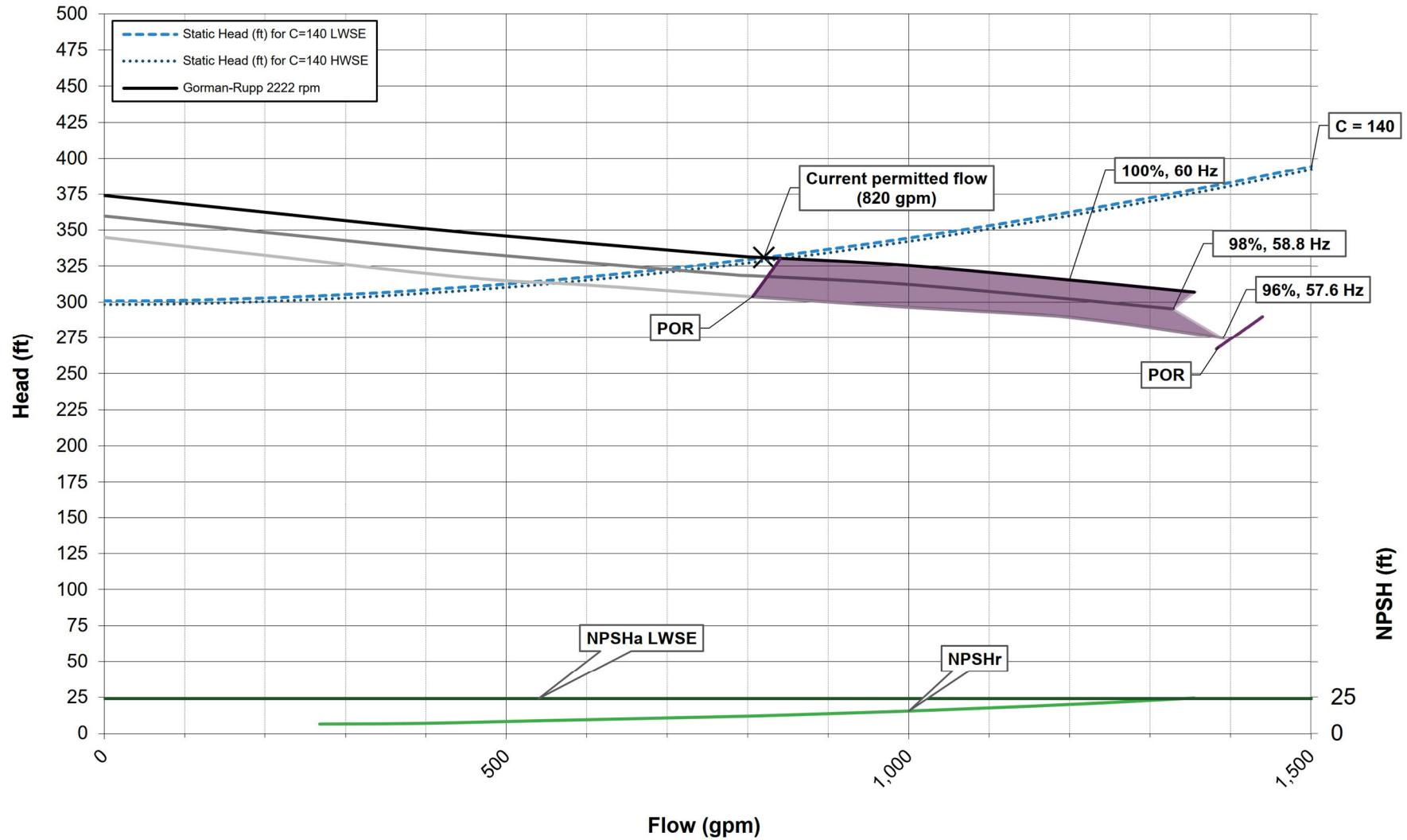
Figure 3.1: Pump Sheaved for Permitted Flow (Current Conditions) – Gorman Rupp 6504E60-B 2222 rpm (1 Pump)
