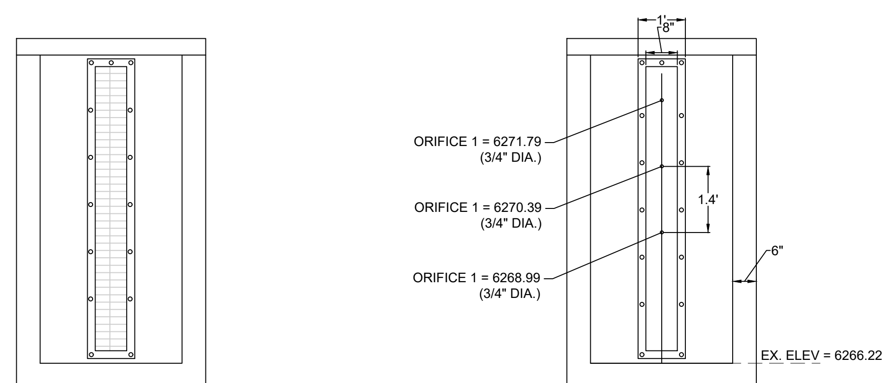
WELL SCREEN SCALE: 1" = 2'
