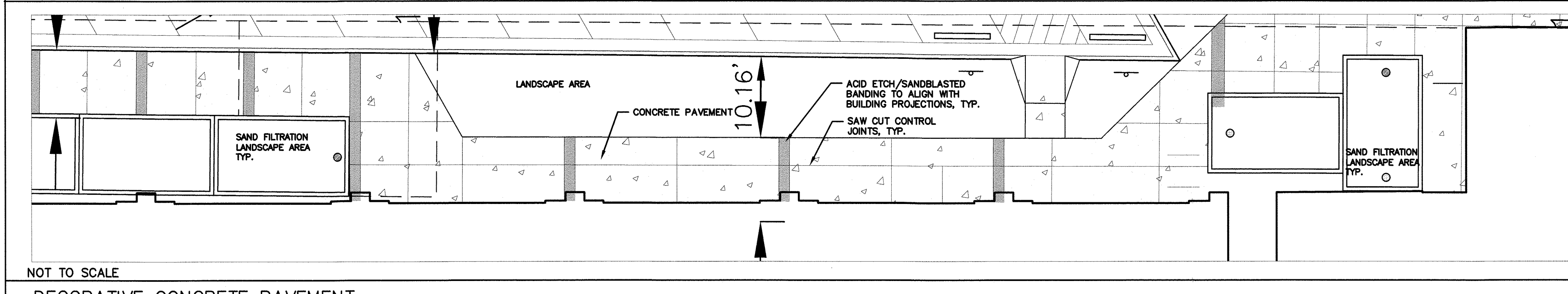
DECORATIVE CONCRETE PAVEMENT
