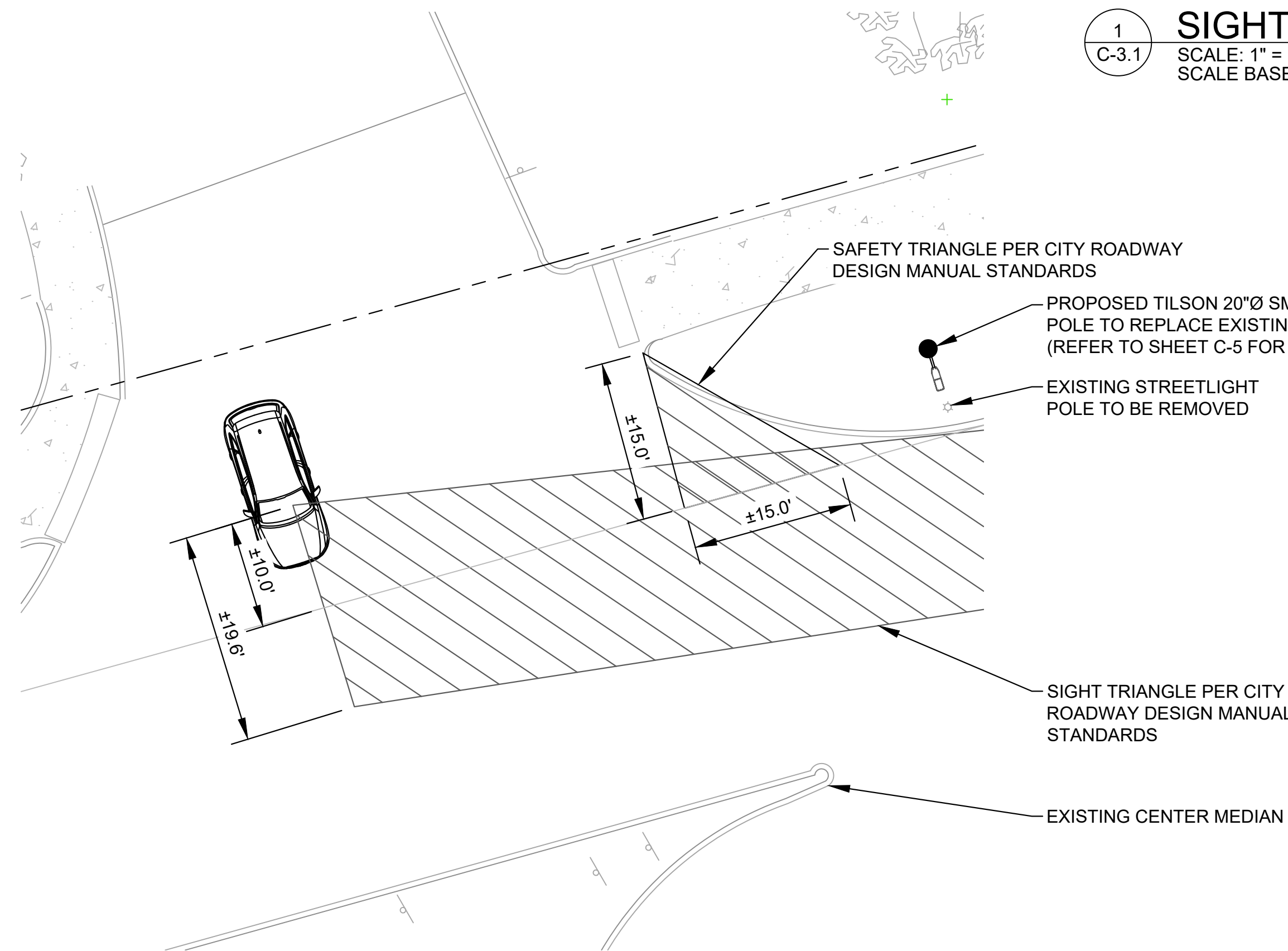
2 C-3.1 ENLARGED SIGHT DISTANCE PLAN SCALE: 1" = 10' SCALE BASED ON 24"X36" ONLY
