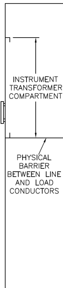
SIDE VIEW
